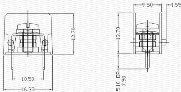
SINGLE WAY TERMINAL (Model: SWT-[C], where C is customized color)
