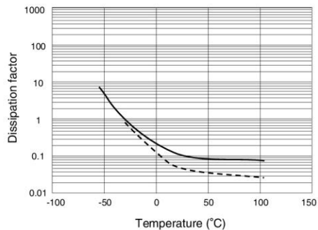
Dissipation factor vs. temperature
