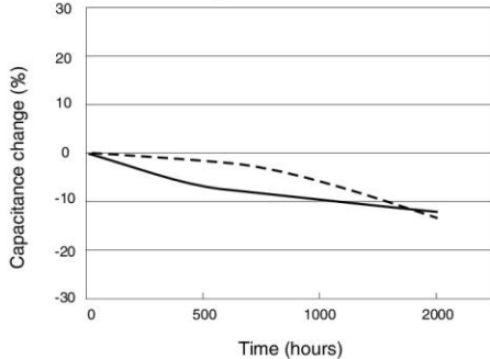
Capacitance change vs. time
