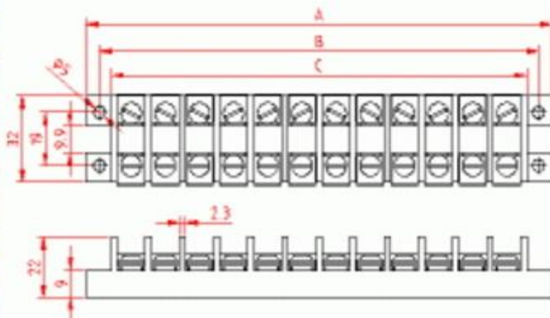
TERMINAL BLOCK 30A OPEN BARRIER TYPE DIMENSION TABLE
