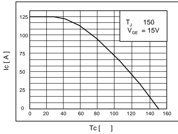
Fig 13. rated Current vs. Case Temperature
